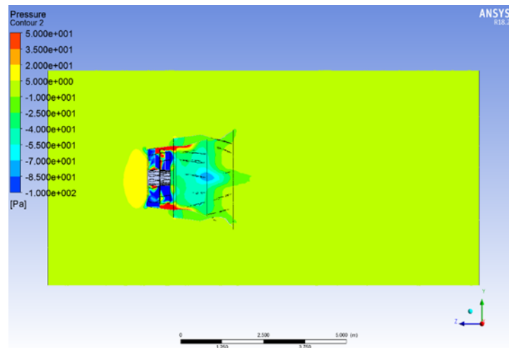
Fig. 8. Pressure contour
