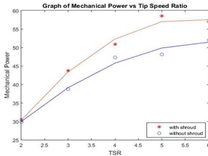
Fig. 5. Comparison on the mechanical power of the wind turbine with and without shroud
