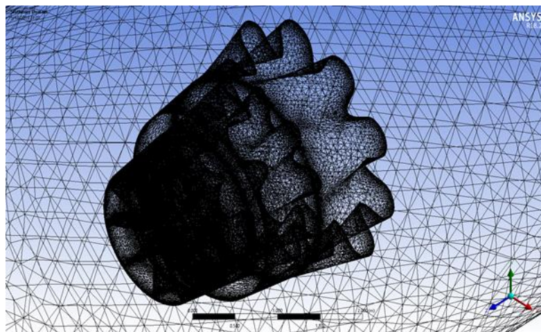
Fig. 3. Edge sizing on the blade and shroud of the jet-engine inspired Wind Turbine
