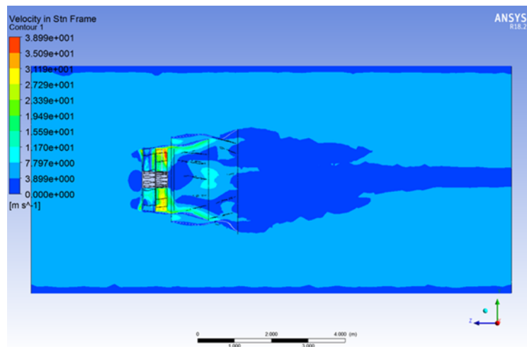
Fig. 9. Velocity contour
