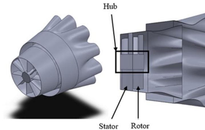
Fig. 1. Isometric and side view of the jet-engine inspired Wind Turbine concept [13]
