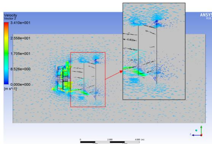
Fig. 7. Vector contour on the wind turbine to capture the swirl formation
