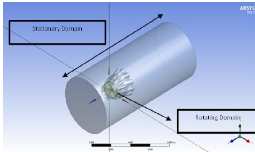
Fig. 2. Numerical domain on the jet-engine inspired Wind Turbine
