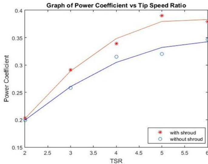
Fig. 6. Comparison on the power coefficient of the wind turbine with and without shroud
