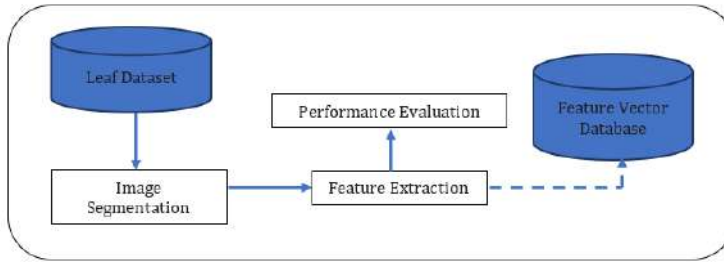
Figure 2: Herb leaves features extraction process flow.
