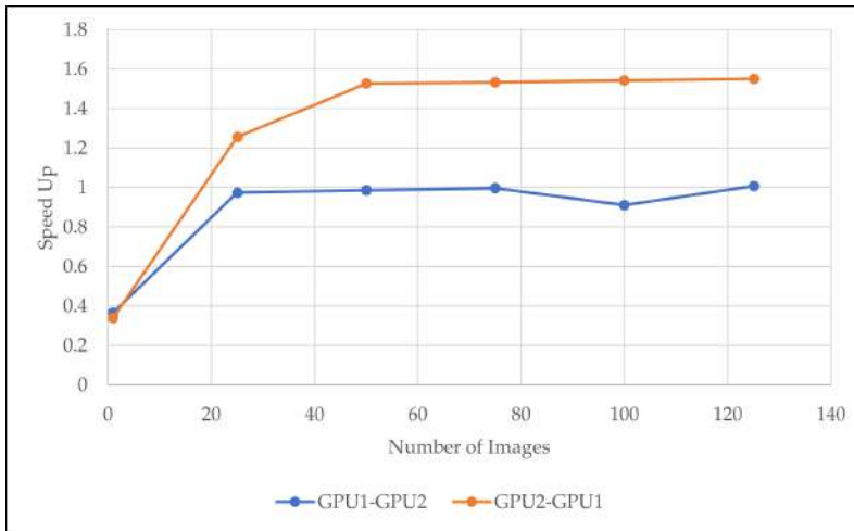
Figure 6: The speedup of two different architectures using two GPUs for different number of images for kernel 1 and kernel 2.
