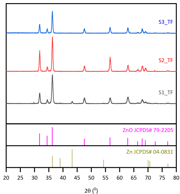
Figure 5. XRD patterns of the ZnO thin films annealed at different oxidation temperatures
