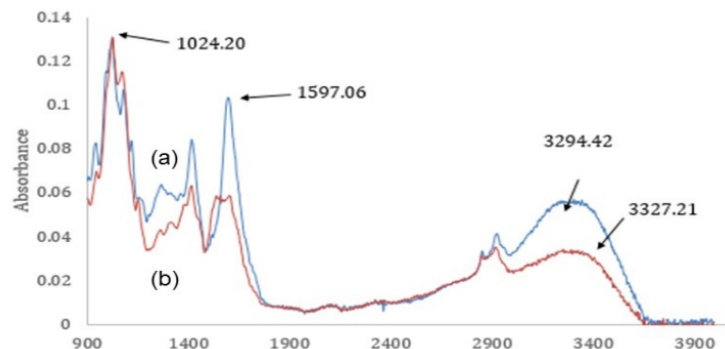
Figure 3. Fourier-transform infrared (FTIR) spectroscopy of immobilized MAG1 in (a) alginate, labeled in blue, and (b) alginate-chitosan, labeled in red.
