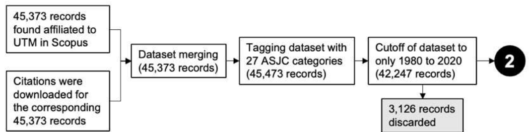
Figure 1. Dataset preparation.
