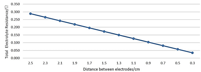
Figure 6. Electrolyte Resistance with varying electrode distances
