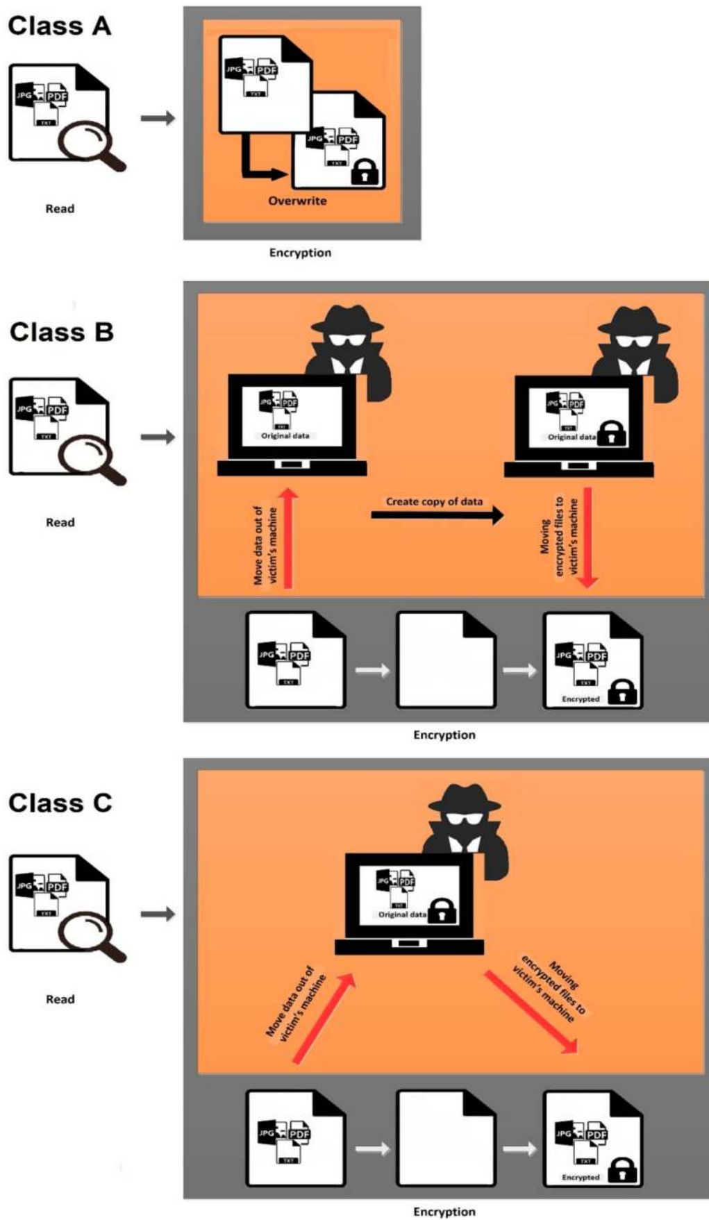
Figure 3. Ransomware attack behavior.
