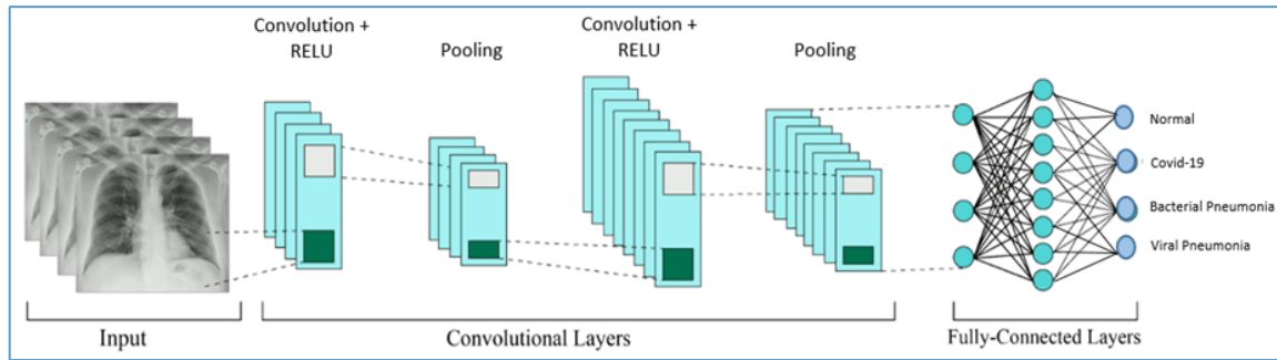
Fig. 3. Overall CNN model's architecture
