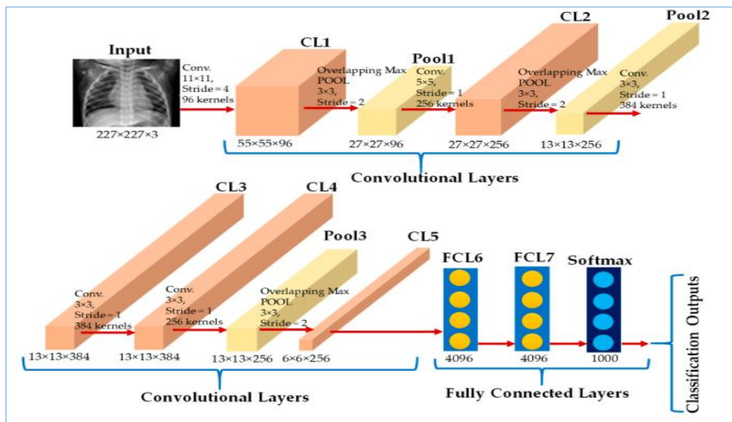
Fig. 4. AlexNet Structure [34]
