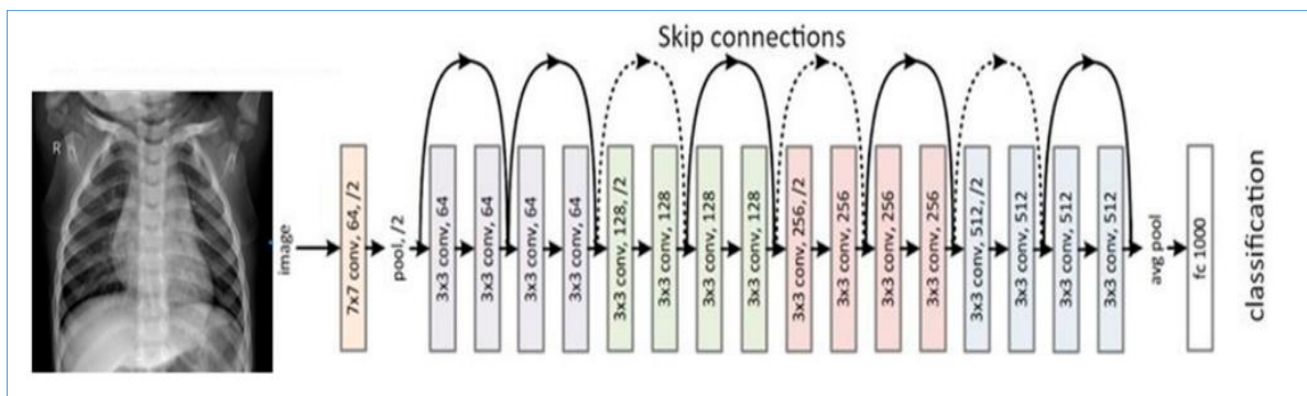
Fig. 6. ResNet-18 Structure [38]
