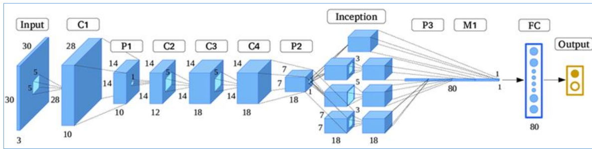
Fig. 7. GoogleNet Structure [40]
