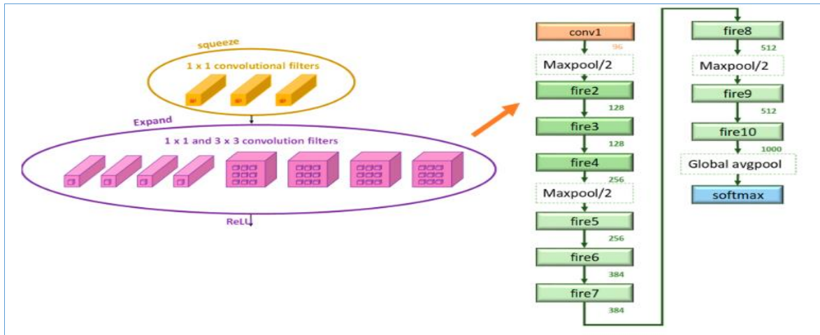
Fig. 5. SqueezeNet Structure [37]
