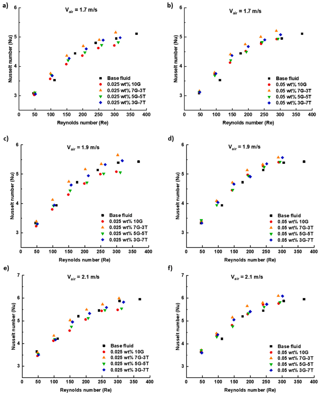
Fig. 7. Effect of hybrid mixing ratio on Nusselt number of 0.025 wt% and 0.05 wt% nanocoolant. a), b) 1.7 m/s; c), d) 1.9 m/s; e), f) 2.1 m/s.
