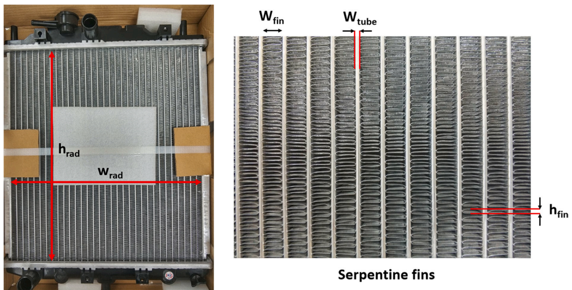
Fig. 3. Structure of crossflow radiator and type of fins used in the current study.
