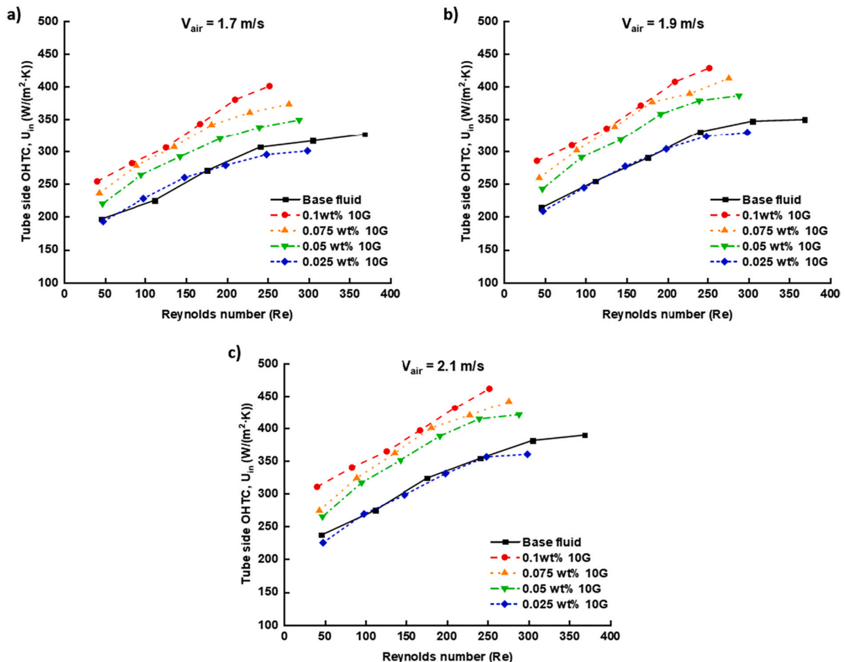
Fig. 9. Effect of nanoparticles concentration on tube side OHTC of 10G nanocoalant at different air velocities. a) 1.7 m/s; b) 1.9 m/s; c) 2.1 m/s.
