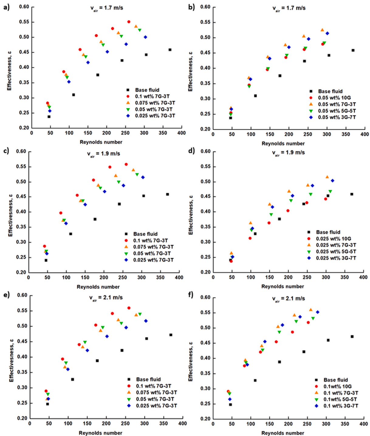
Fig. 12. Different effects on the effectiveness of radiator. a), c), e) Nanoparticle's concentration; b), d), f) Mixing ratio.
