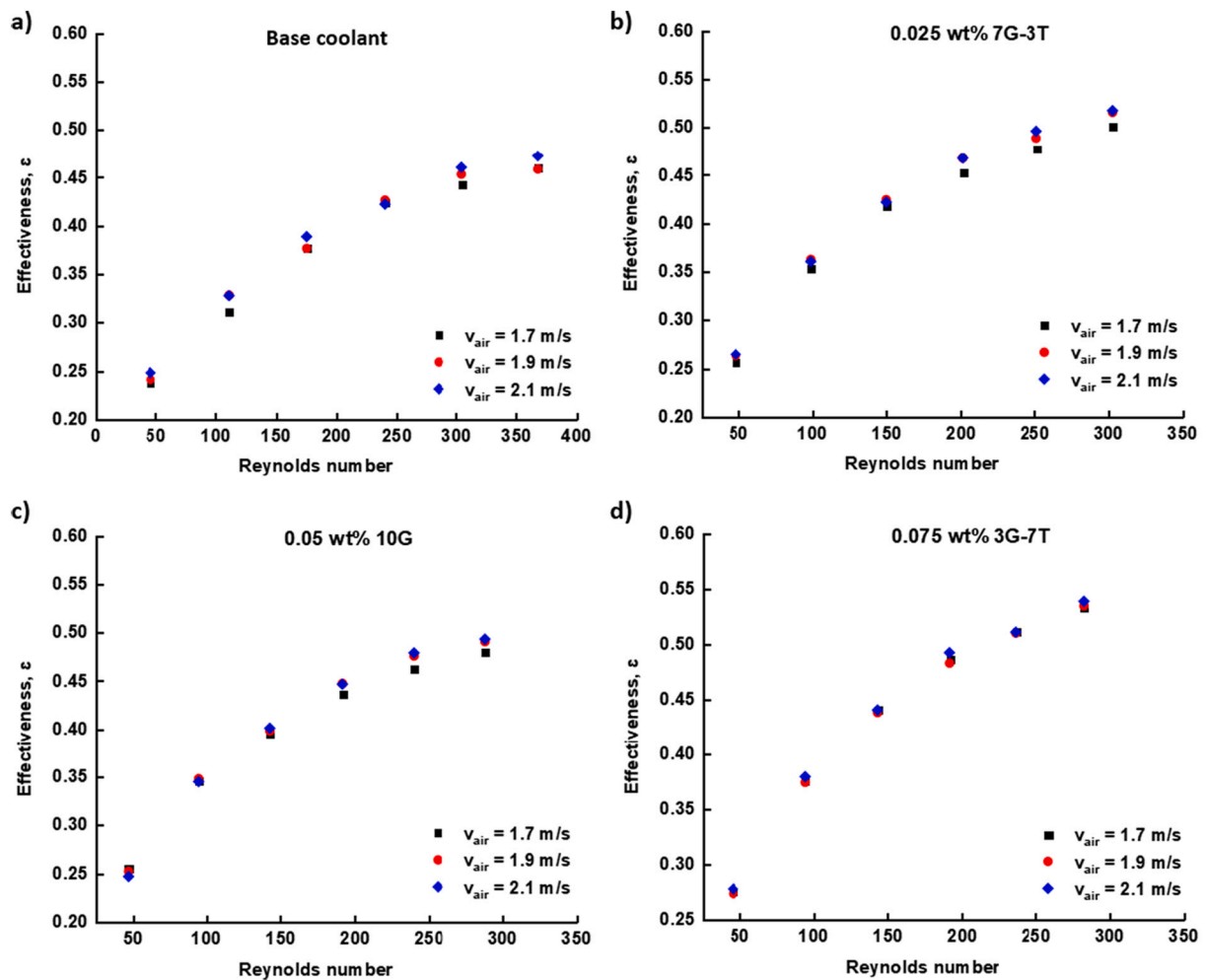
Fig. 13. Effect of air velocity on the effectiveness of radiator.
