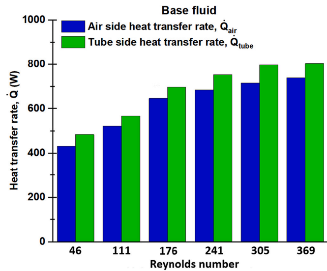
Fig. 4. Verification of experimental data by judging heat balance error at different Reynolds numbers.
