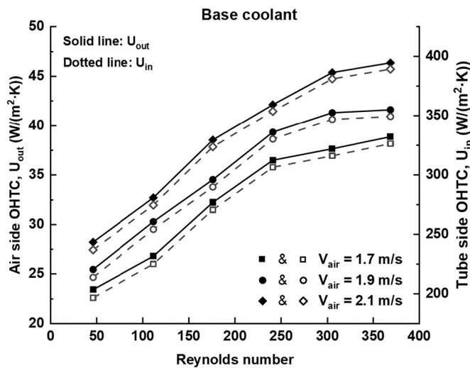
Fig. 8. Airside and tube side OHTC of base coolant at different air velocities.
