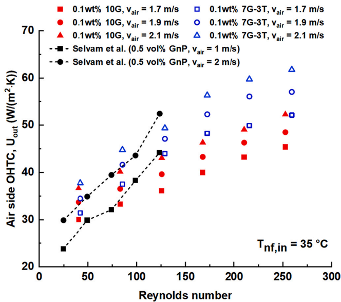
Fig. 11. Comparison of airside OHTC with the past study.
