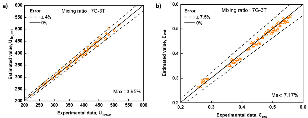
Fig. 14. Comparison of estimated heat transfer performance against experimental data. a) Tube side OHTC b) Effectiveness of radiator.
