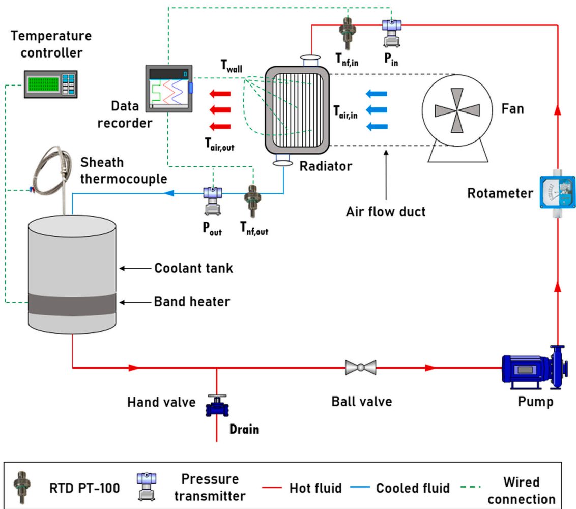
Fig. 2. The schematic diagram for the heat transfer test rig.
