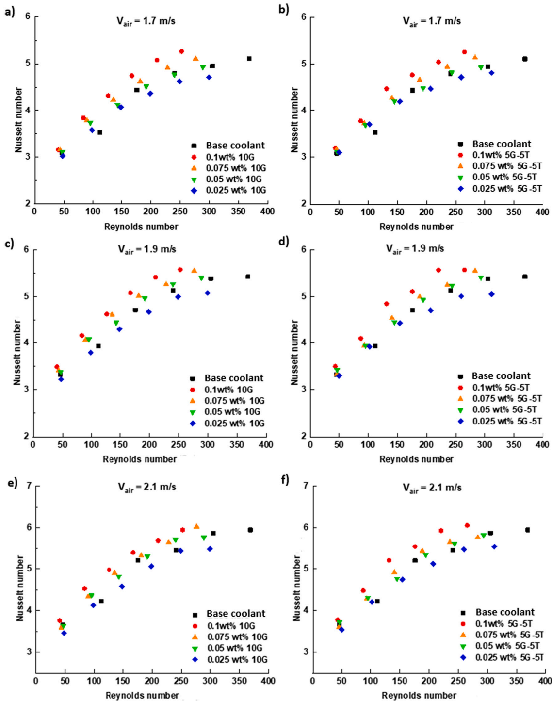
Fig. 6. Effect of nanoparticles concentration on Nusselt number on 10G and 5G-5T nanocoolant. a), b) 1.7 m/s; c), d) 1.9 m/s; e), f) 2.1 m/s.
