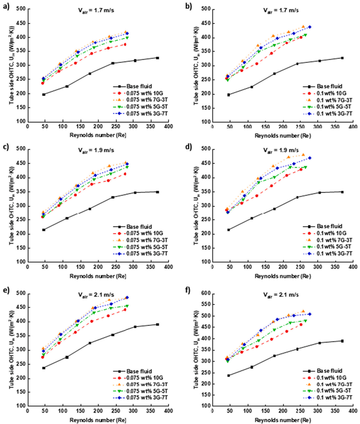
Fig. 10. Effect of mixing ratio on tube side OHTC. a), c), e) 0.075 wt% b), d), f) 0.1 wt%.
