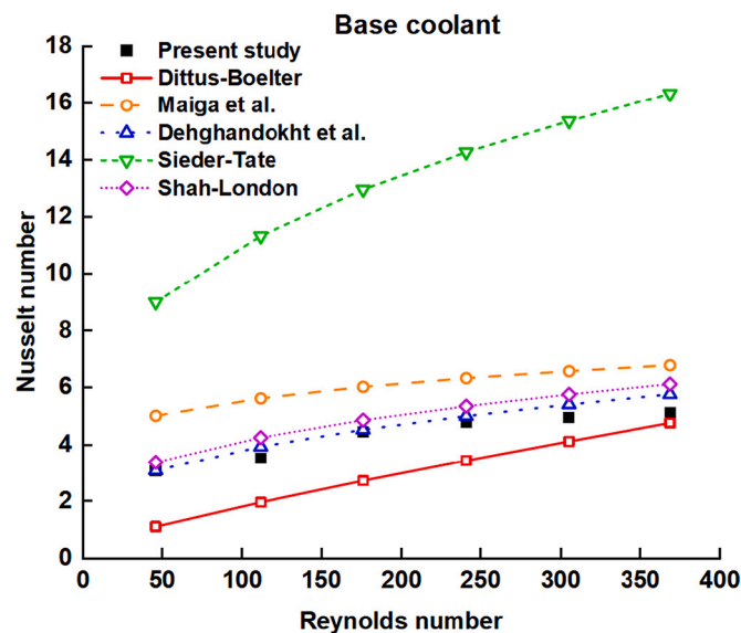
Fig. 5. Nusselt number of base coolants obtained from experiment and computed using different correlations at an air velocity of 1.7 m/s.
