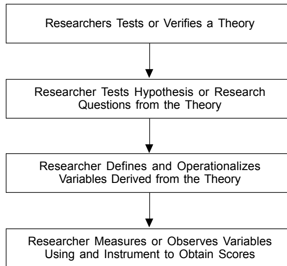
Figure 2 The deductive approach (Source: Adopted from Creswell, 2003: 125)
