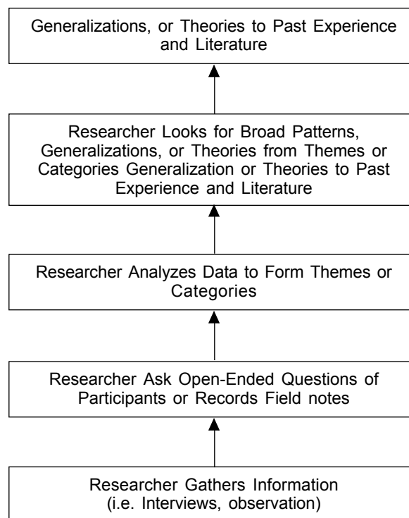
Figure 1 The inductive logic (Source: Adopted from Cresswell, 2003: 132)
